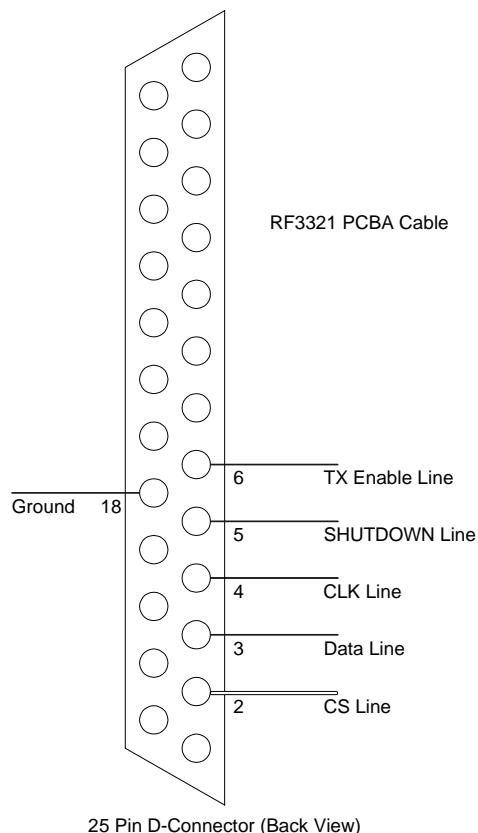
Figure 3. Cable Configuration
