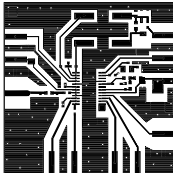
Evaluation Board Layout 915MHz Board Size 1.5" x 1.5"
