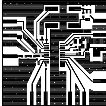
Evaluation Board Layout 433MHz Board Size 1.5" x 1.5"
