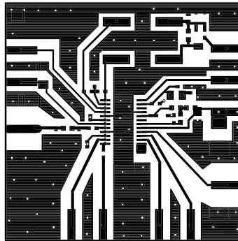
Evaluation Board Layout 868MHz Board Size 1.5" x 1.5"
