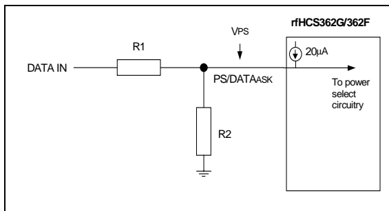
FIGURE 6-5: EXAMPLE ASK POWER SELECT CIRCUIT
