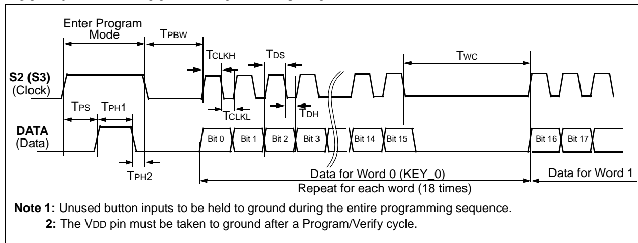
FIGURE 5-1: PROGRAMMING WAVEFORMS
