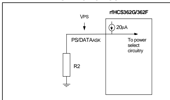
FIGURE 6-6: EXAMPLE FSK POWER SELECT CIRCUIT
