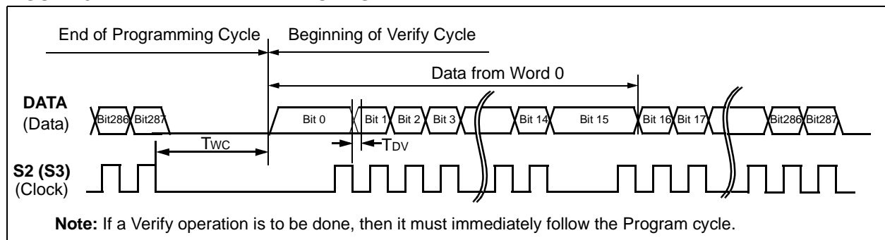
FIGURE 5-2: VERIFY WAVEFORMS
