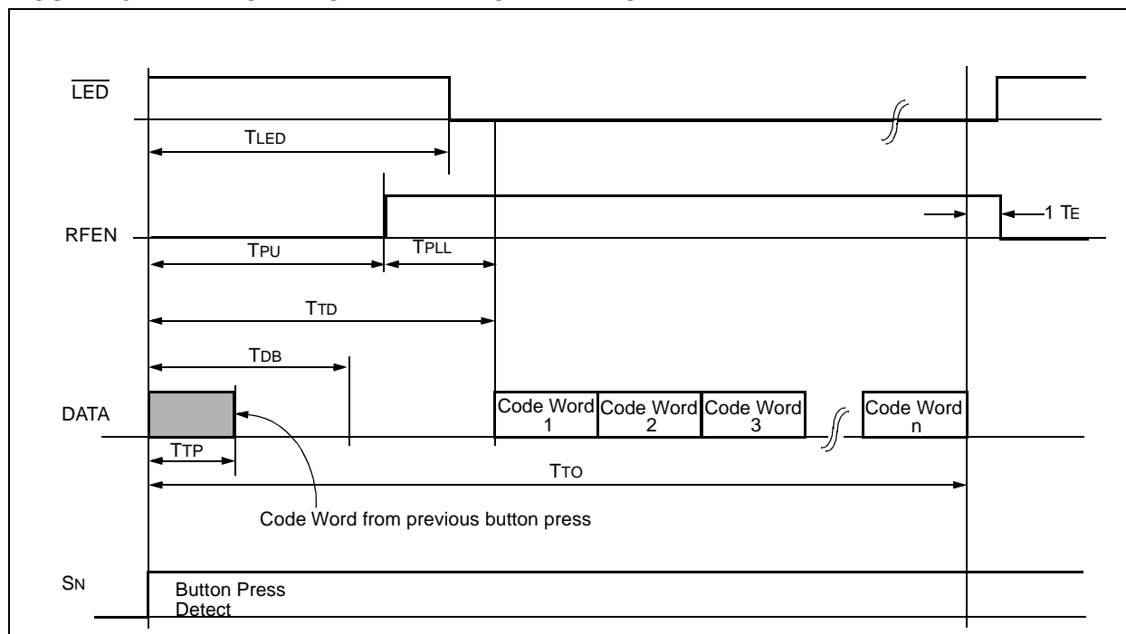
FIGURE 10-1: POWER-UP AND TRANSMIT TIMING
