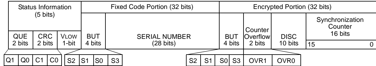
FIGURE 3-6: CODE WORD DATA FORMAT
