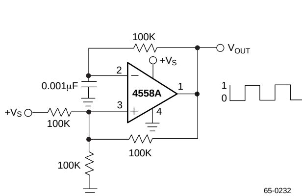
Figure 22. Squarewave Oscillator
