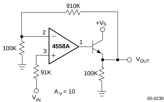
Figure 20. Power Amplifier
