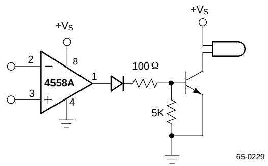
Figure 19. Lamp Driver
