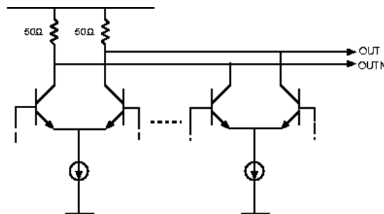
Figure 5. The RDA012V1 equivalent output circuit
