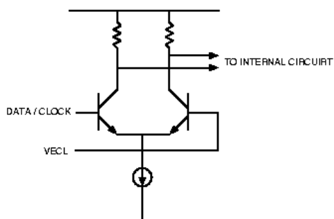
Figure 2. The internal data and clock input circuit of the RDA012V1 DAC
