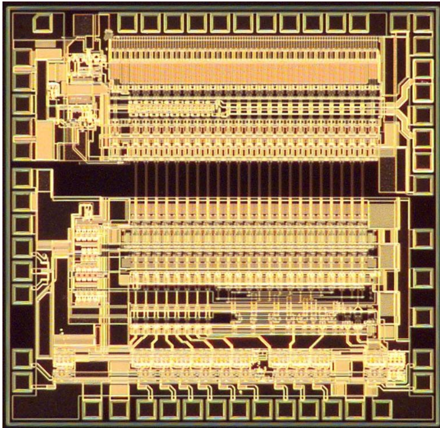
Figure 7. RDA012V1 Die Photo, after scribe, 2.740mm x 2.650mm
