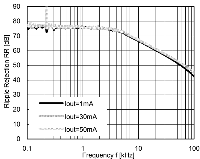
R1160X081X ECO=H V IN =1.8VDC+0.2Vp-p, C IN ; none, C OUT =tantal2.2μF
