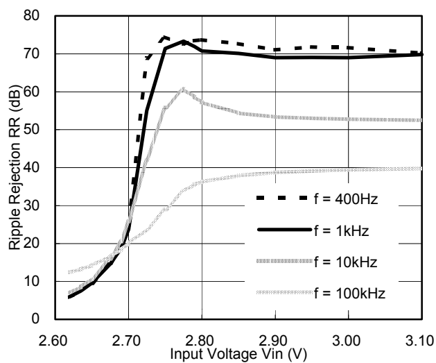
R1160X261X Ripple 0.2Vp-p I out =50mA C IN ; none C OUT =Tantal2.2μF
