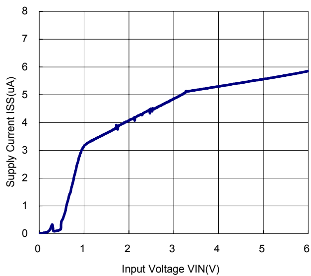
R1160X331X ECO=L
