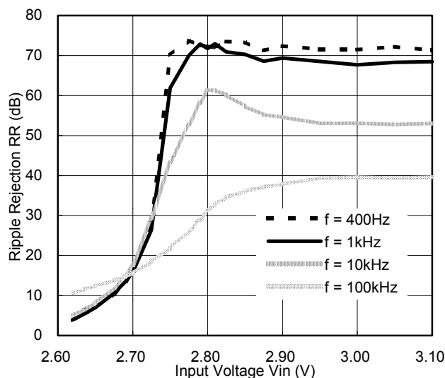
R1160X261X Ripple 0.2Vp-p I out =50mA C IN ; none C OUT =Tantal2.2μF
