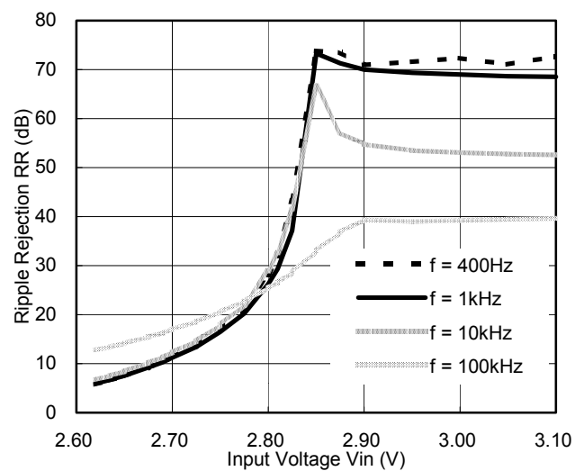
R1160X261X Ripple 0.5Vp-p I out =50mA C IN ; none C OUT =Tantal2.2μF
