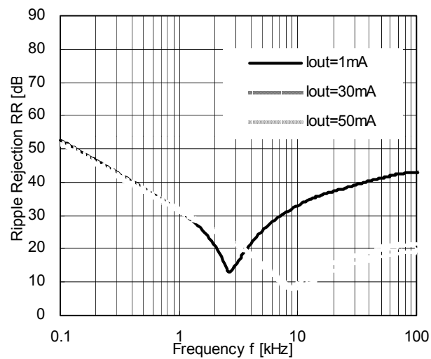
R1160X081X ECO=L V IN =1.8VDC+0.2Vp-p, C IN ; none, C OUT =tantal2.2μF
