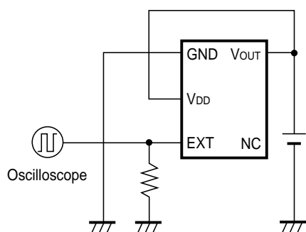
Test Circuit3
