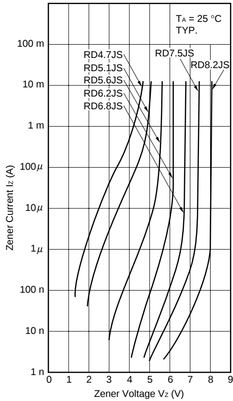
Fig. 3 I_Z - V_Z CHARACTERISTICS
