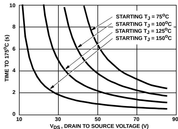
FIGURE 23. TIME TO 175^{\circ}\text{C} IN CURRENT LIMITING (HEATSINK THERMAL RESISTANCE = 10^{\circ}\text{C/W} ) (HEATSINK THERMAL CAPACITANCE = 1.0\text{J/}^{\circ}\text{C} )
