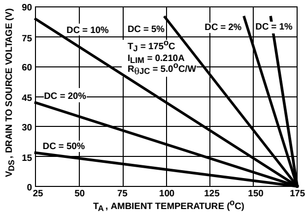
FIGURE 21. MAXIMUM V_{DS} vs AMBIENT TEMPERATURE IN CURRENT LIMITING. (HSTR = 80^{\circ}\text{C/W} )
