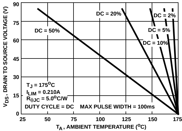
FIGURE 19. MAXIMUM V_{DS} vs AMBIENT TEMPERATURE IN CURRENT LIMITING. (HSTR = 10^{\circ}\text{C/W} )
