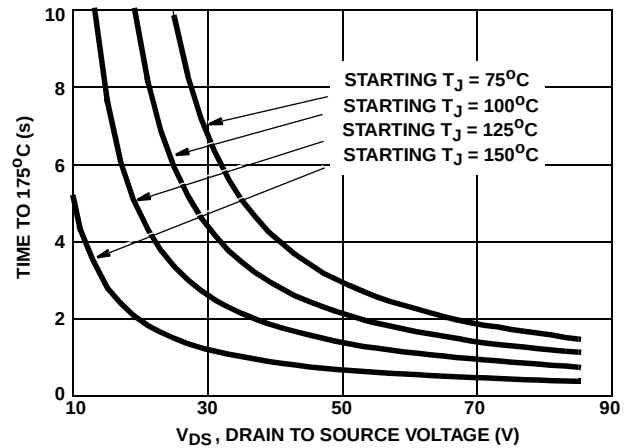
FIGURE 22. TIME TO 175^{\circ}\text{C} IN CURRENT LIMITING (HEATSINK THERMAL RESISTANCE = 25^{\circ}\text{C/W} ) (HEATSINK THERMAL CAPACITANCE = 0.5\text{J/}^{\circ}\text{C} )
