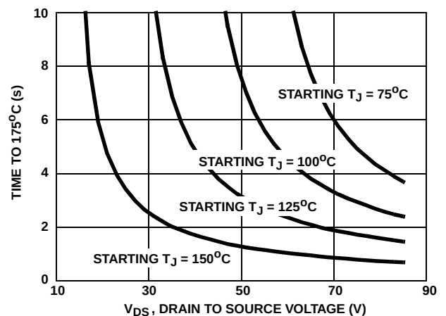
FIGURE 24. TIME TO 175^{\circ}\text{C} IN CURRENT LIMITING (HEATSINK THERMAL RESISTANCE = 5^{\circ}\text{C/W} ) (HEATSINK THERMAL CAPACITANCE = 2.0\text{J/}^{\circ}\text{C} )
