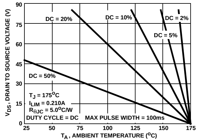
FIGURE 20. MAXIMUM V_{DS} vs AMBIENT TEMPERATURE IN CURRENT LIMITING. (HSTR = 25^{\circ}\text{C/W} )
