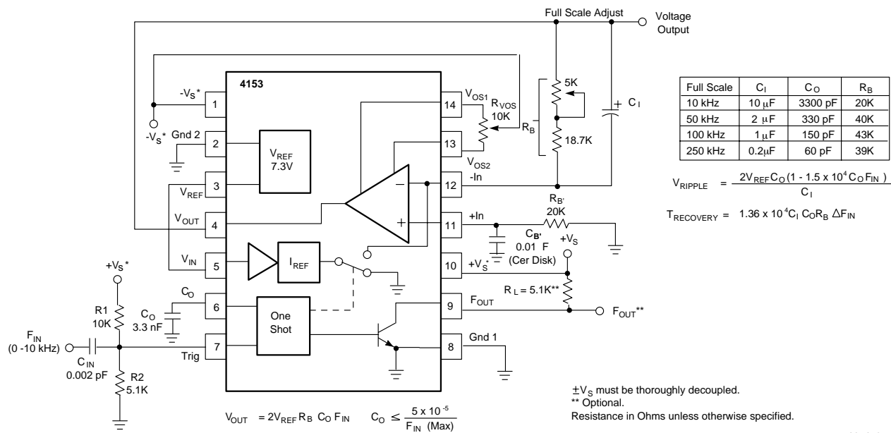
Figure 2. Frequency-to-Voltage Converter
