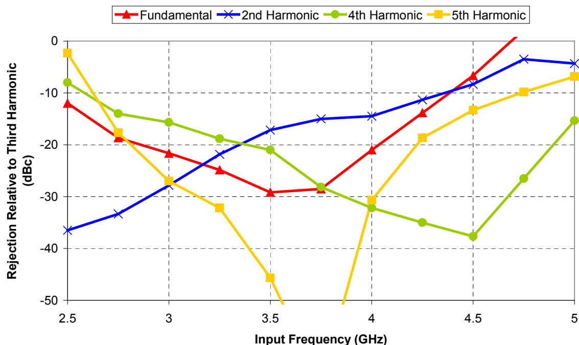
RMWT04001, 4 to 12 GHz Tripler, Typical Performance, Chip Bonded into 50 ohm Test Fixture
