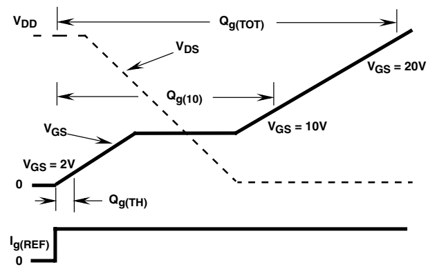
FIGURE 19. GATE CHARGE WAVEFORM
