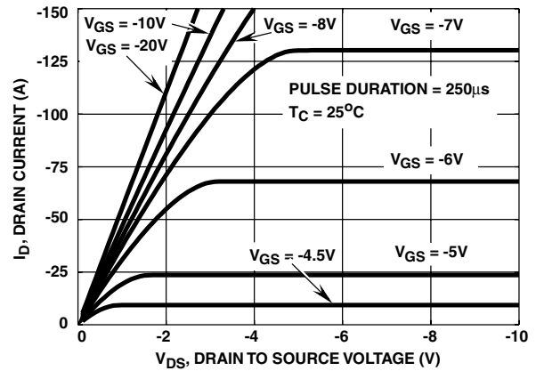
FIGURE 7. SATURATION CHARACTERISTICS
