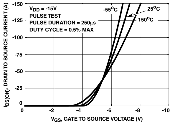
FIGURE 8. TRANSFER CHARACTERISTICS
