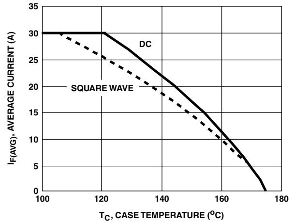
FIGURE 4. CURRENT DERATING CURVE
