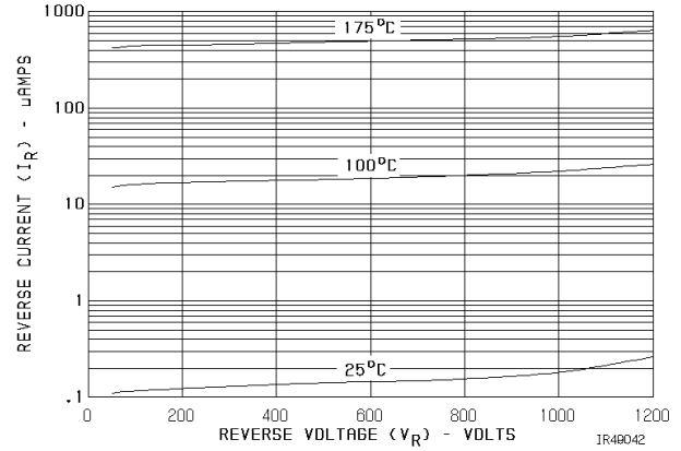
FIGURE 4. TYPICAL REVERSE CURRENT vs VOLTAGE
