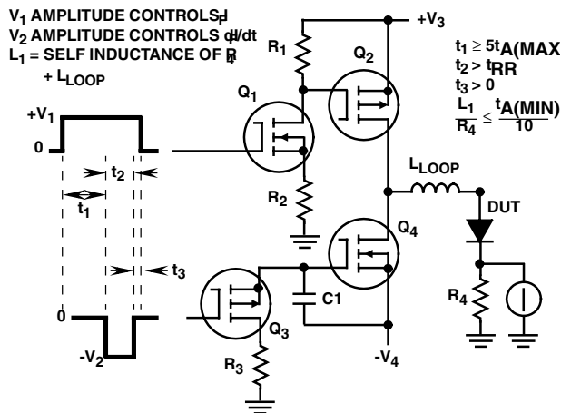
FIGURE 1. t_{RR} TEST CIRCUIT
