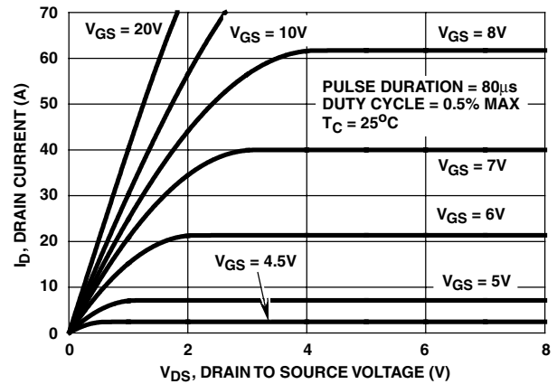
FIGURE 7. SATURATION CHARACTERISTICS
