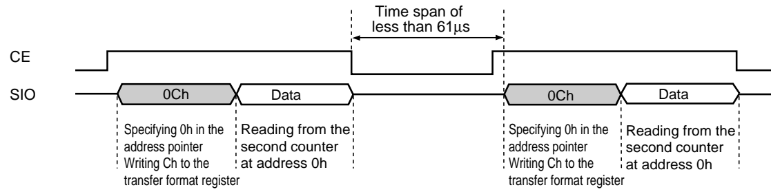
Bad Example (3) (Where a time span of less than 61µs is left between the adjacent processes of reading time data)
