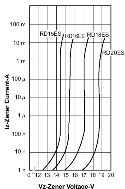
Figure 3. Zener current vs. zener voltage
