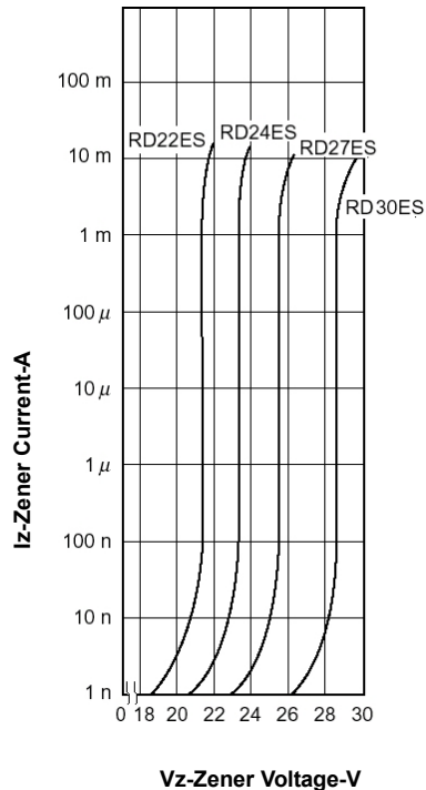
Figure 4. Zener current vs. zener voltage
