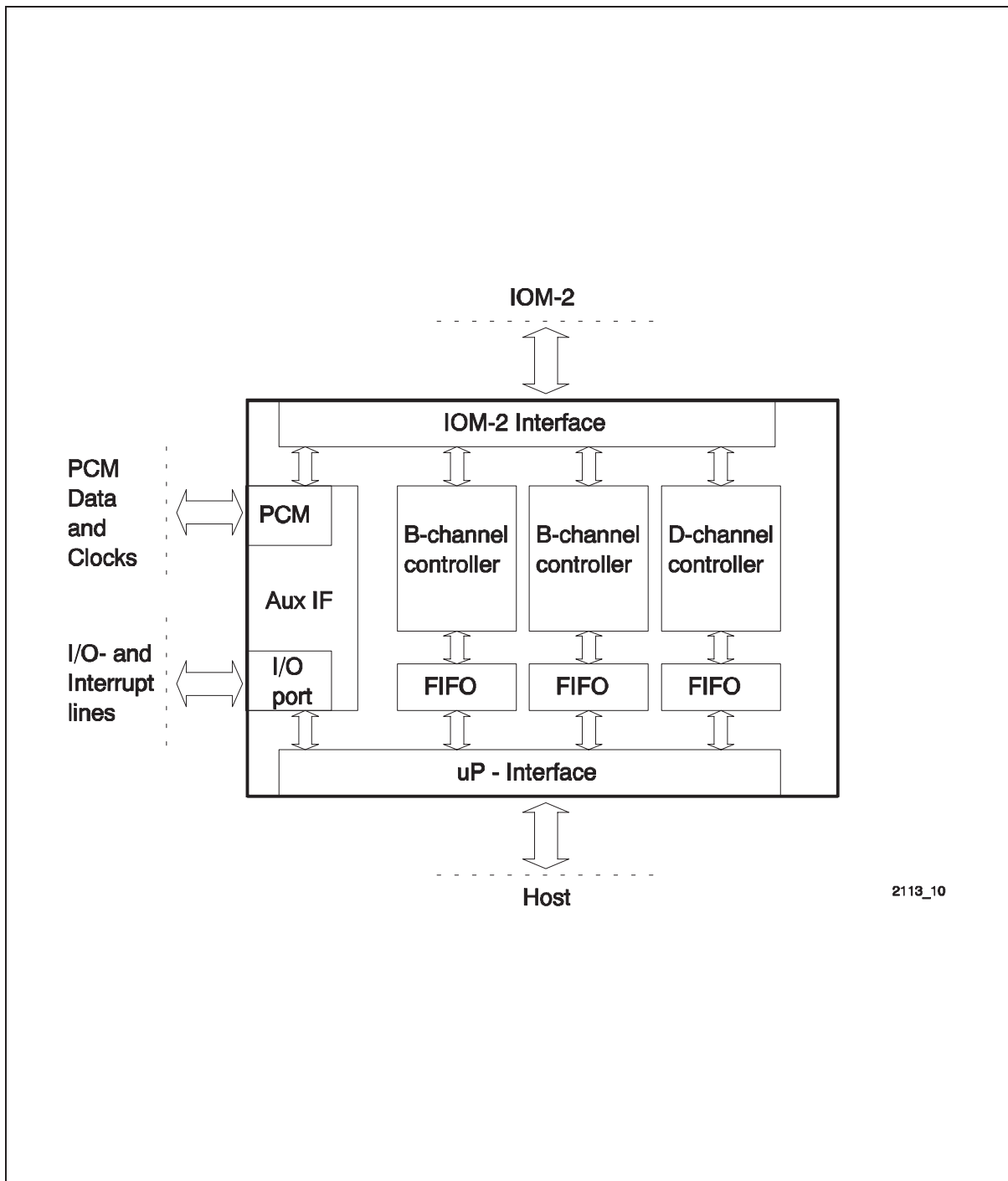
Figure 3 Block Diagram
