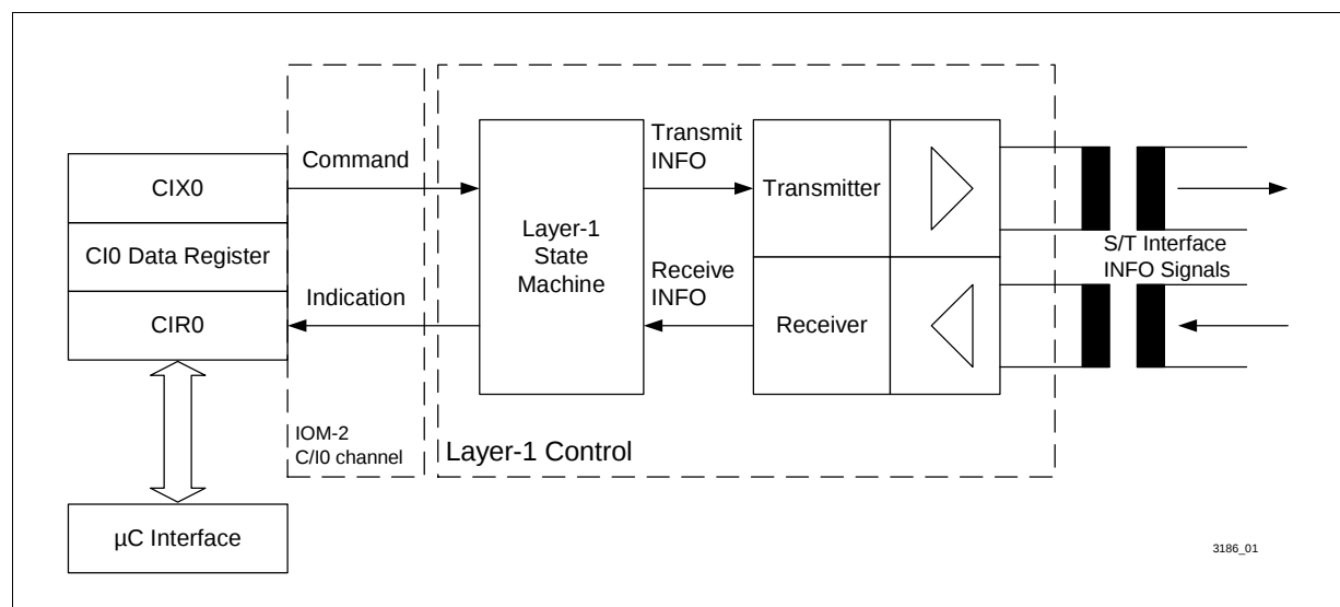
Figure 30 Layer-1 Control
