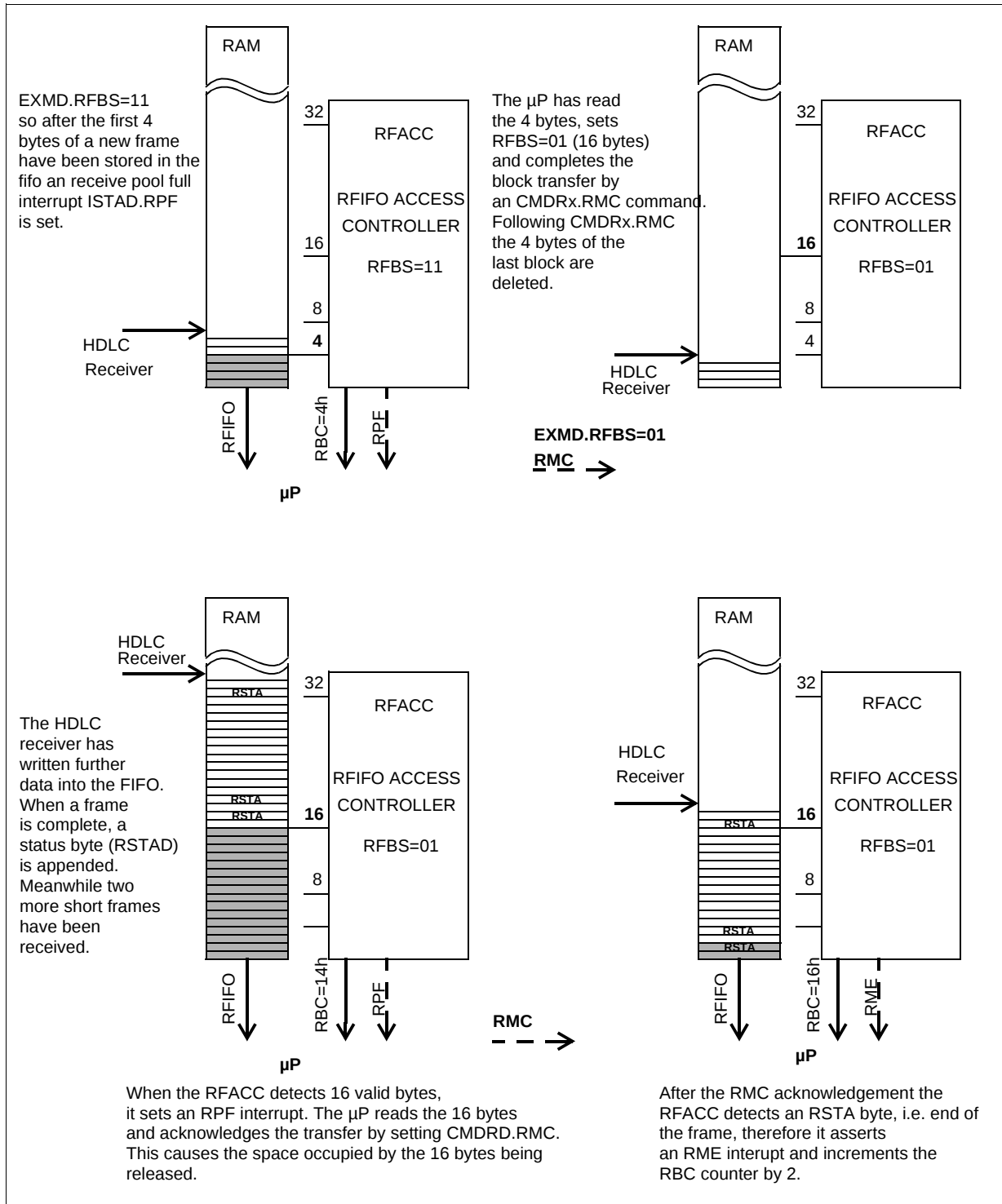
Figure 59 RFIFO Operation
