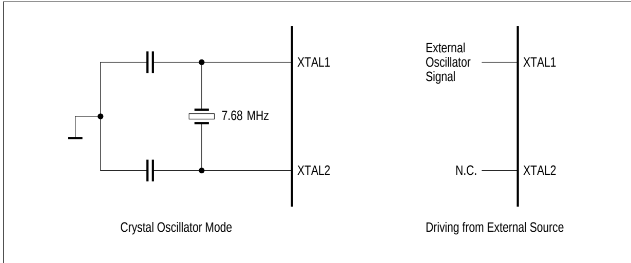
Figure 69 Oscillator Circuits
