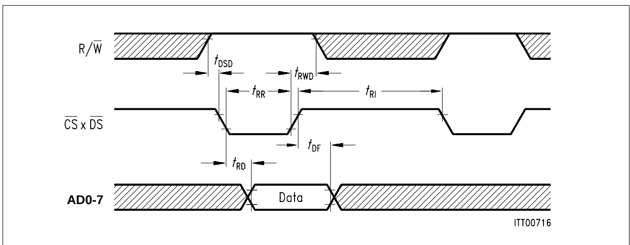
Figure 78 Microprocessor Read Timing
