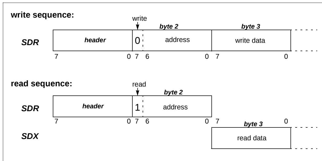
Figure 6 Serial Control Interface Timing
