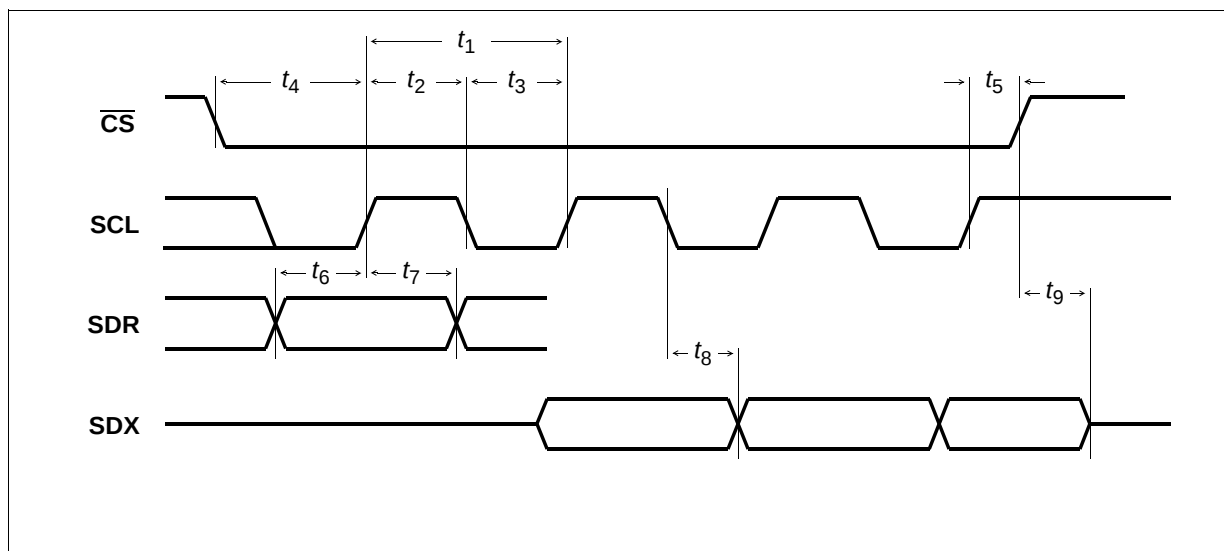
Figure 73 SCI Interface
