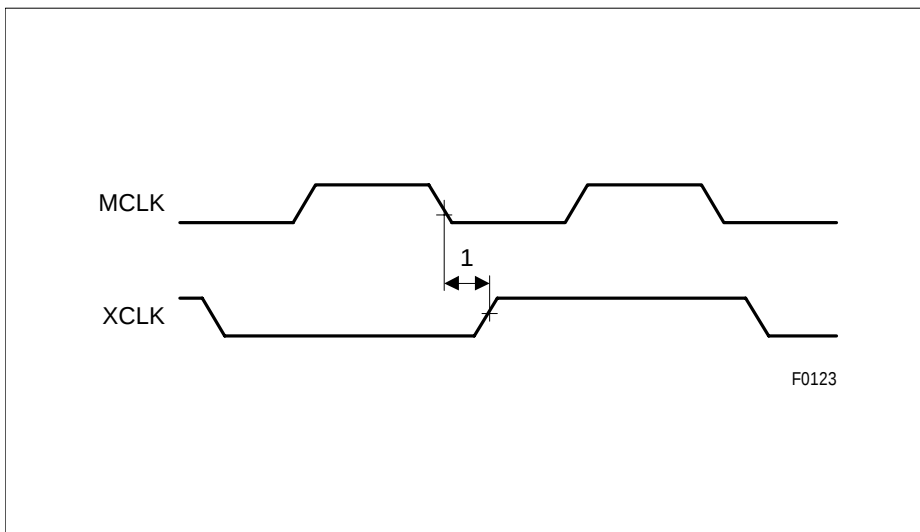
Figure 96 XCLK Timing
