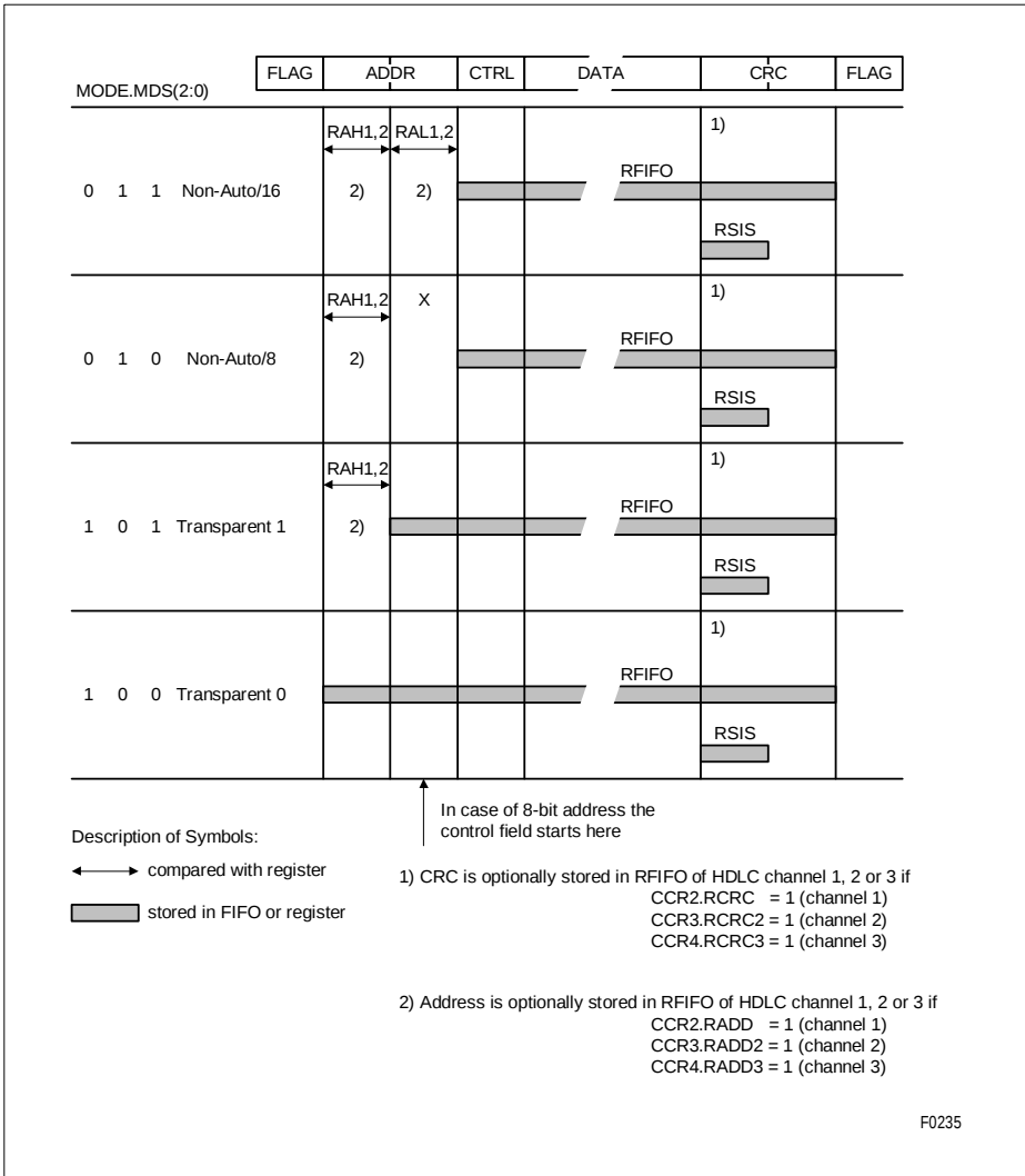
Figure 74 HDLC Receive Data Flow
