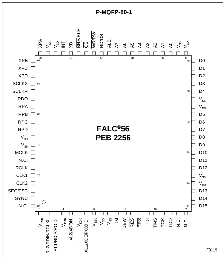
Figure 4 Pin Configuration
