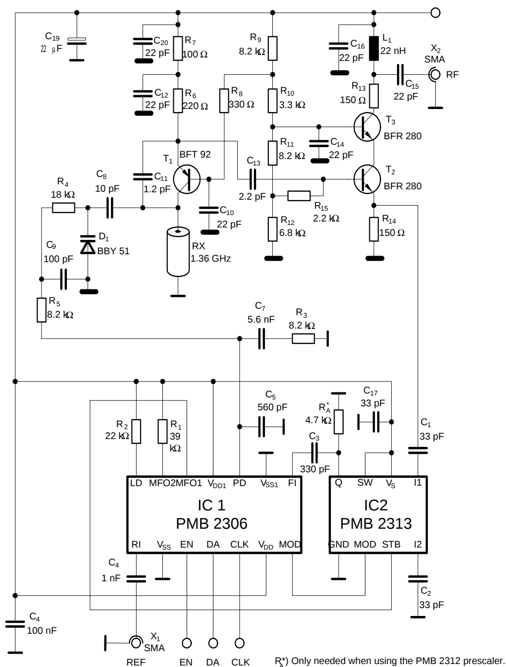
Circuit Diagram
