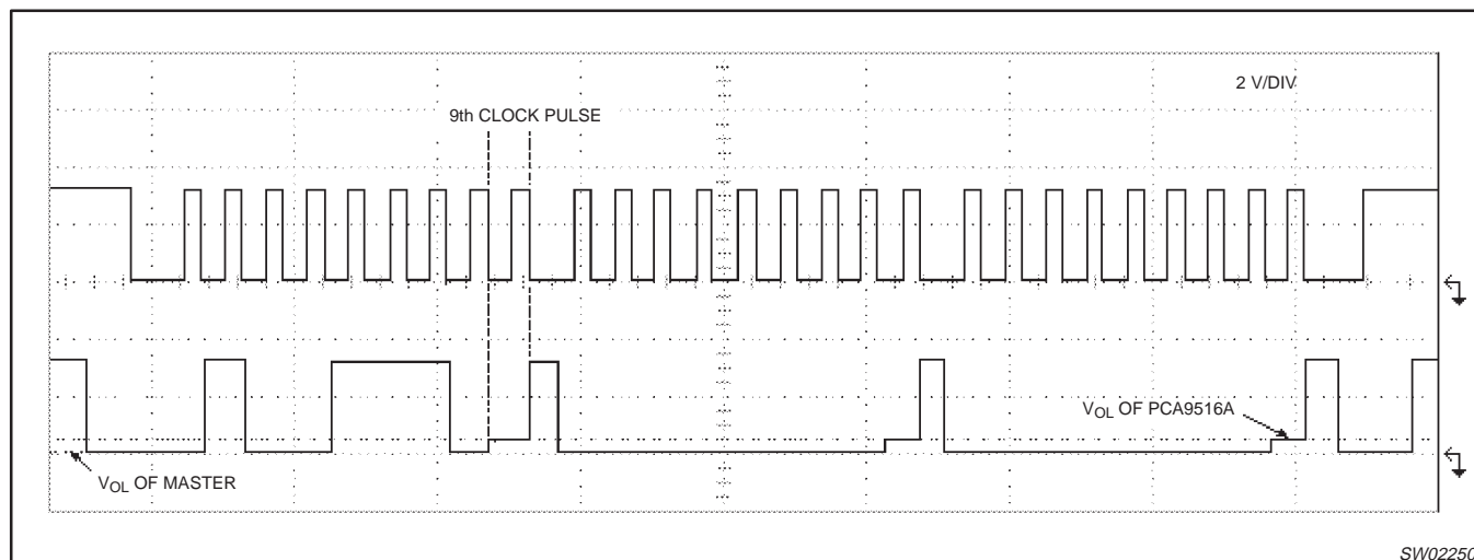
Figure 5. Bus 0 waveform
