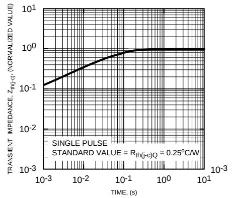
TRANSIENT THERMAL IMPEDANCE CHARACTERISTICS (Each IGBT)
