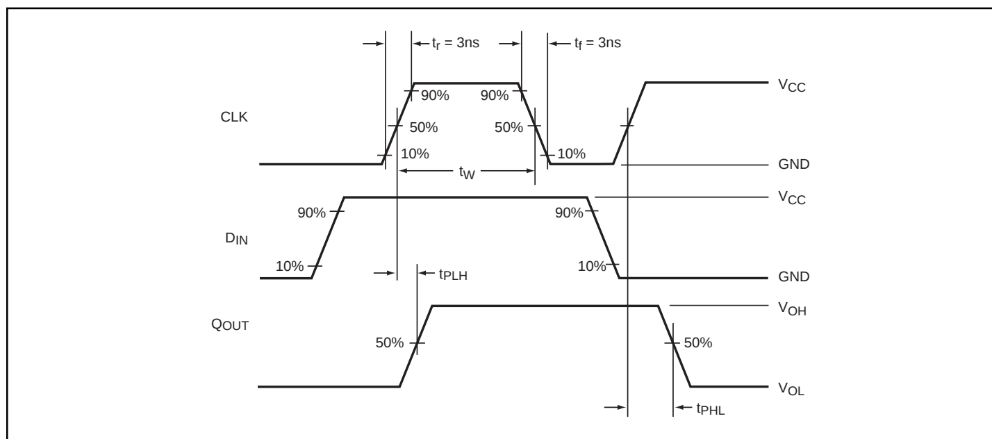
Figure 3. AC Waveforms
