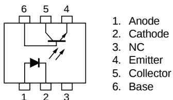
PS2621, PS2621L
