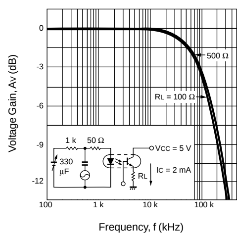
FREQUENCY RESPONSE
