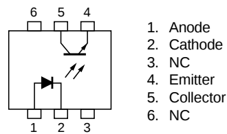
PS2622, PS2622L
