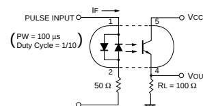
PS2606
