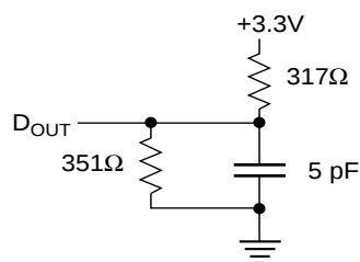
Figure 2. Output Load Equivalent (for TLZCE, tHZCE, tLZWE, tLZOE, tHZOE)
