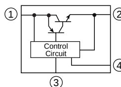
Internal connection diagram
