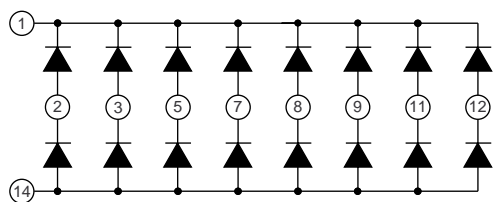
14 DIODE ARRAY NC Pins 4, 6, 10 & 13
