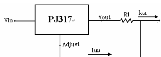
FIGURE 23-CURRENT REGULATOR
