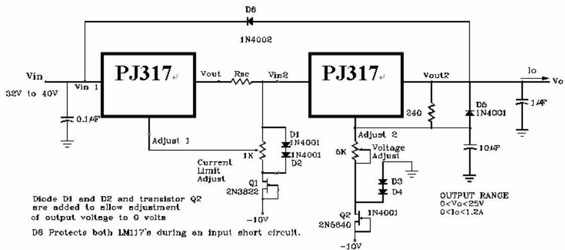
FIGURE 20-ADJUSTABLE CURRENT LIMITER
