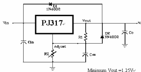
FIGURE 18 - VOLTAGE REGULATOR WITH PROTECTION DIODES
