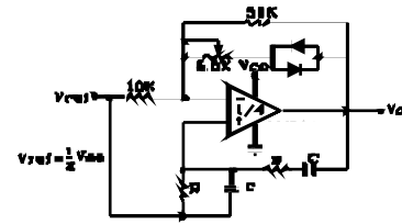
Figure 8. Wien Bridge Oscillator
