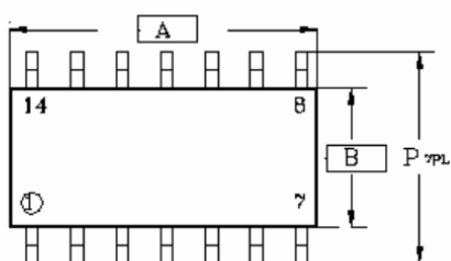
SOP-14
