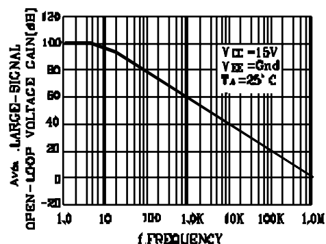
Figure 2. Open-Loop Frequency
