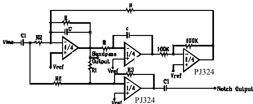
Figure 11. Bi-Quad Filter
