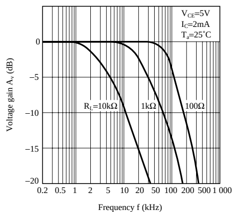
Fig.12 Frequency Response
