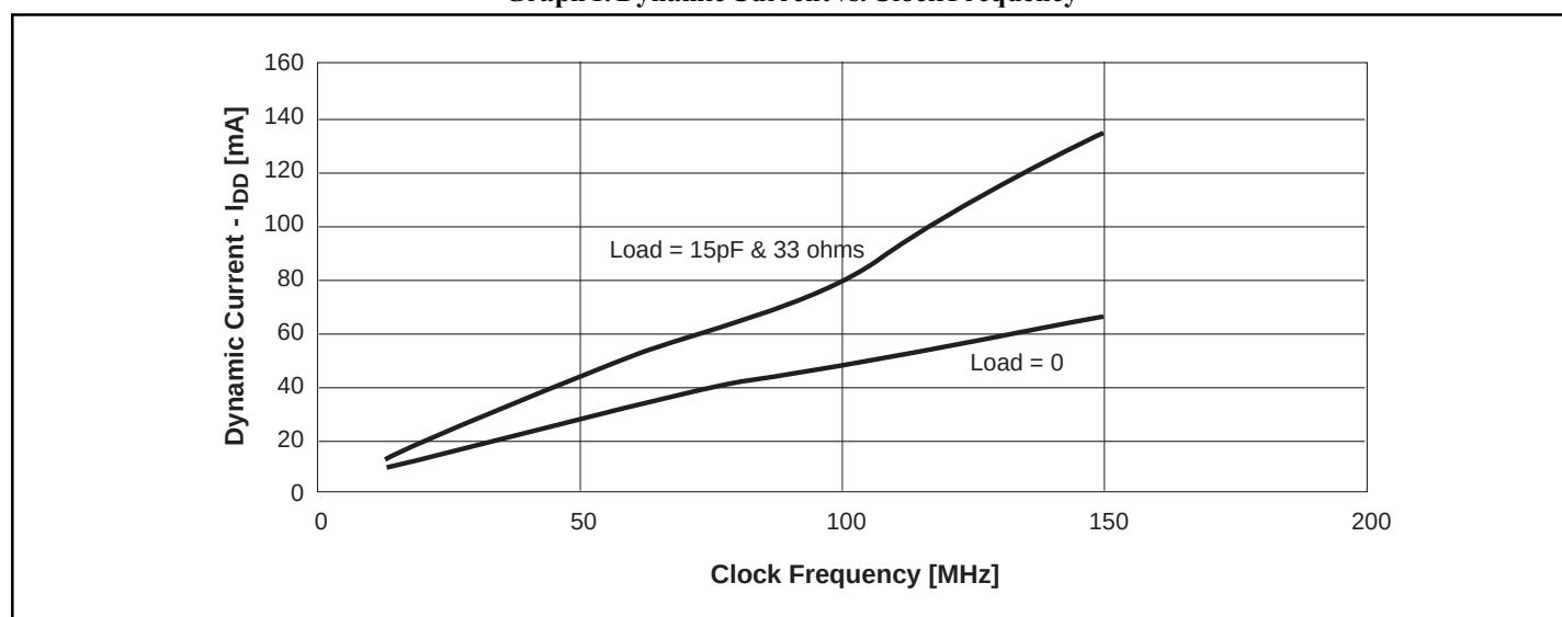
Graph 1. Dynamic Current vs. Clock Frequency
