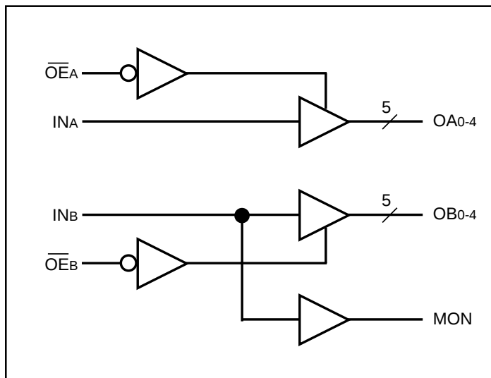
PI49FCT3805 Logic Block Diagram
