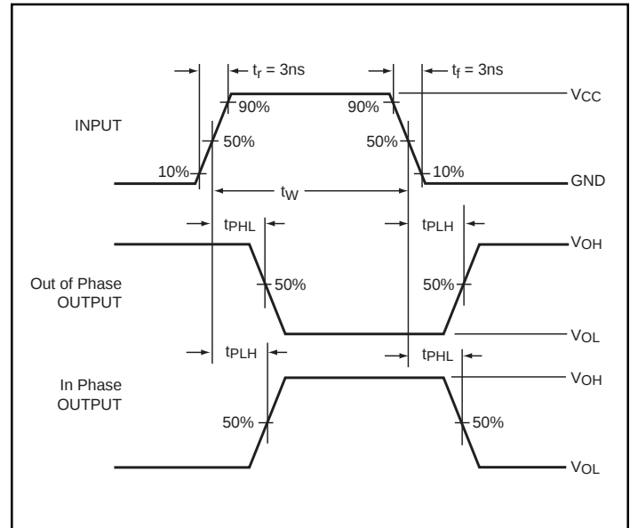
Figure 3. AC Waveforms
