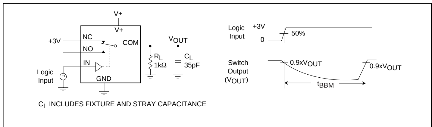
Figure 3. Break-Before-Make Interval
