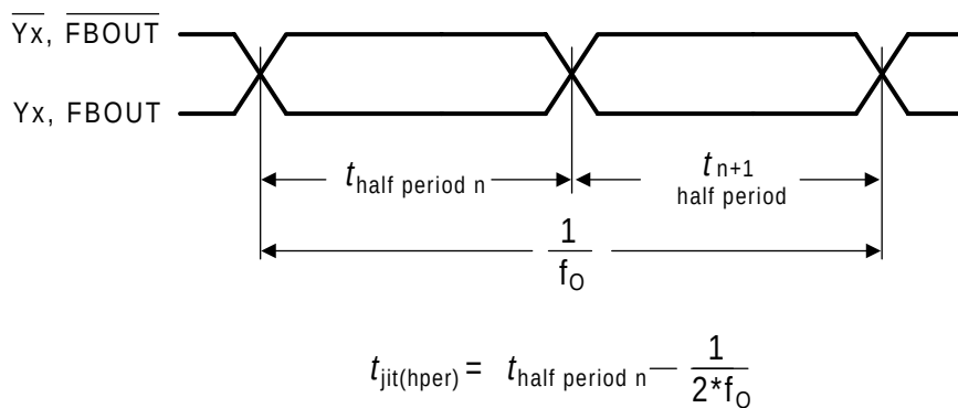
Figure 7. Half-Period Jitter
