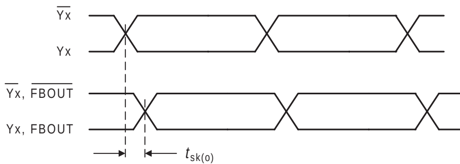
Figure 5. Output Skew
