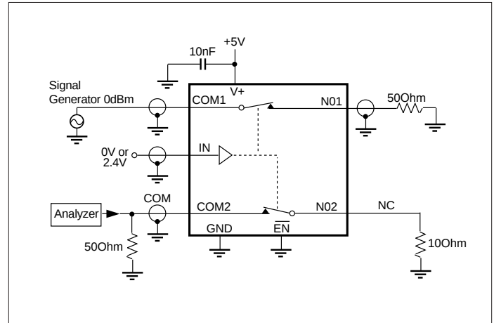
Figure 4. Crosstalk
