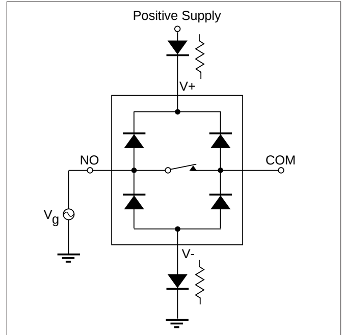
Figure 8. Overvoltage protection is accomplished using two external blocking diodes or two current limiting resistors.
