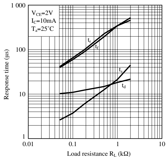
Fig.14 Response Time vs. Load Resistance
