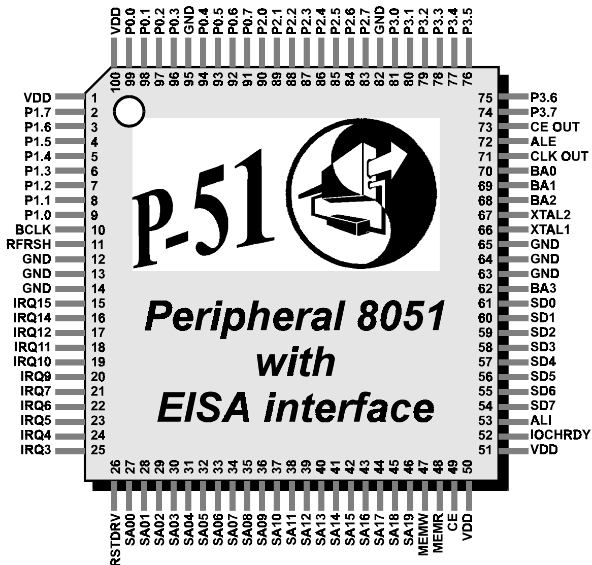
P-51 Pinout Diagram
