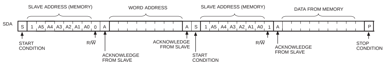
Figure 14. Random Read
