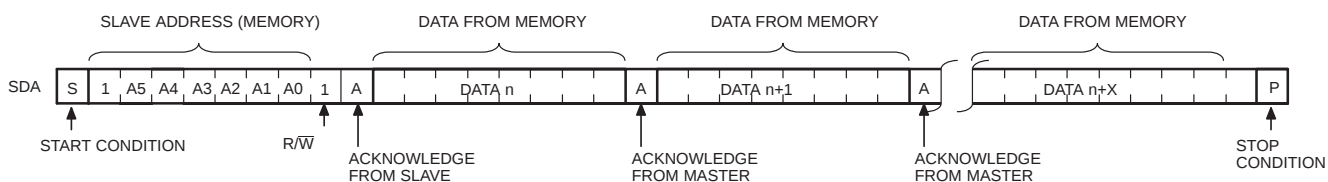
Figure 15. Sequential Read
