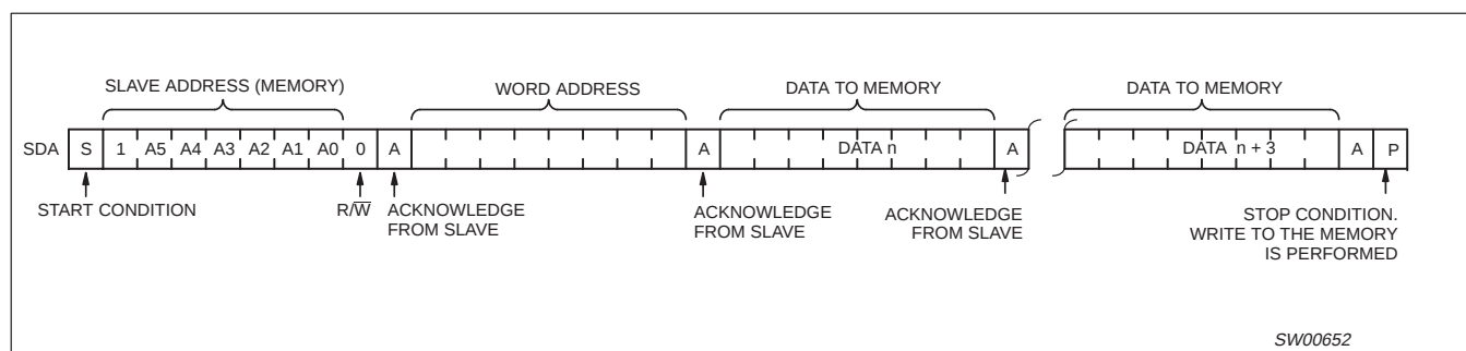
Figure 12. Page Write
