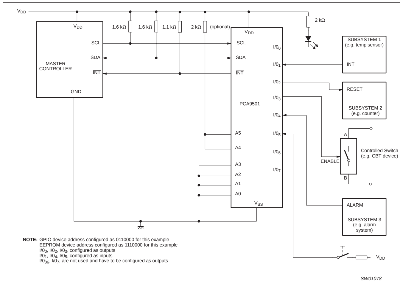
Figure 21. Typical application
