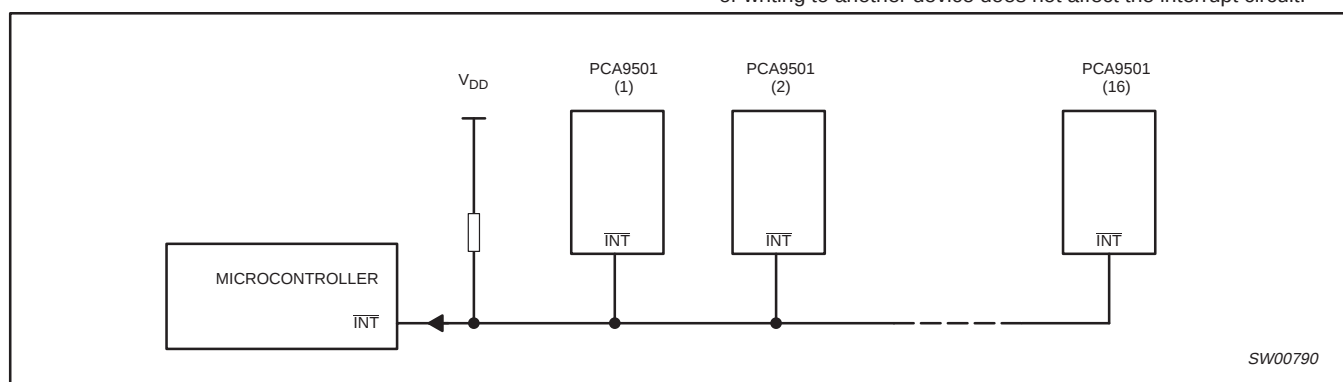
Figure 9. Application of multiple PCA9501s with interrupt
