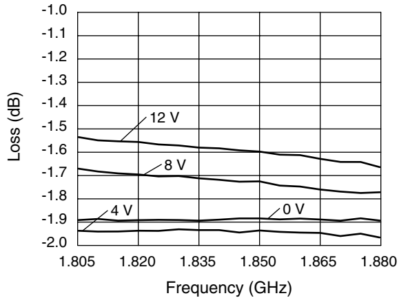
Insertion Loss vs. Frequency and Control Voltage
