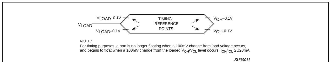
Figure 38. Float Waveform
