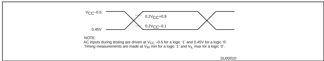
Figure 37. AC Testing Input/Output
