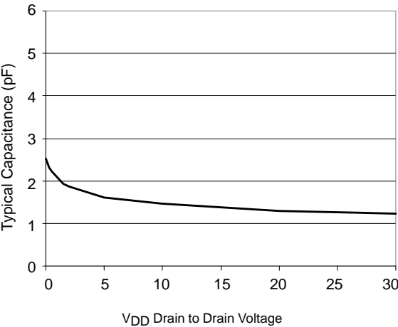
Figure 7. Output Capacitance
