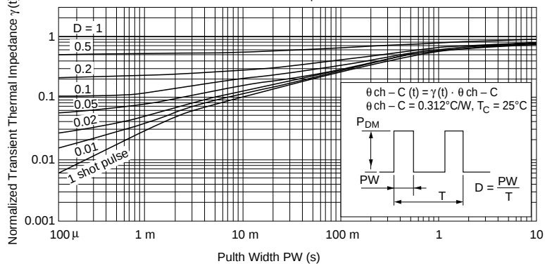
Normalized Transient Thermal Impedance vs. Pulse Width
