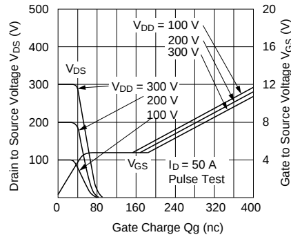
Switching Characteristics
