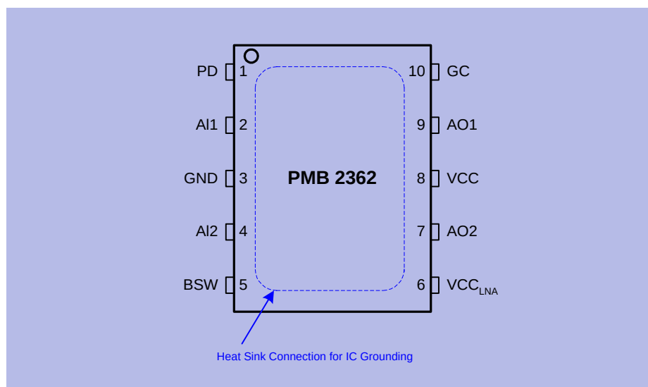
Figure 3-1 Pin Configuration
