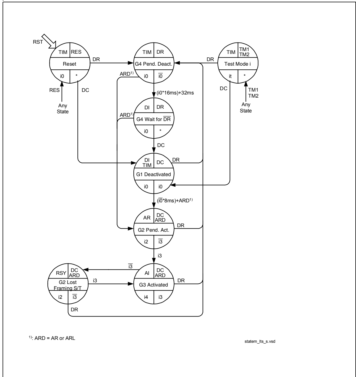
Figure 41 State Machine LT-S Mode
