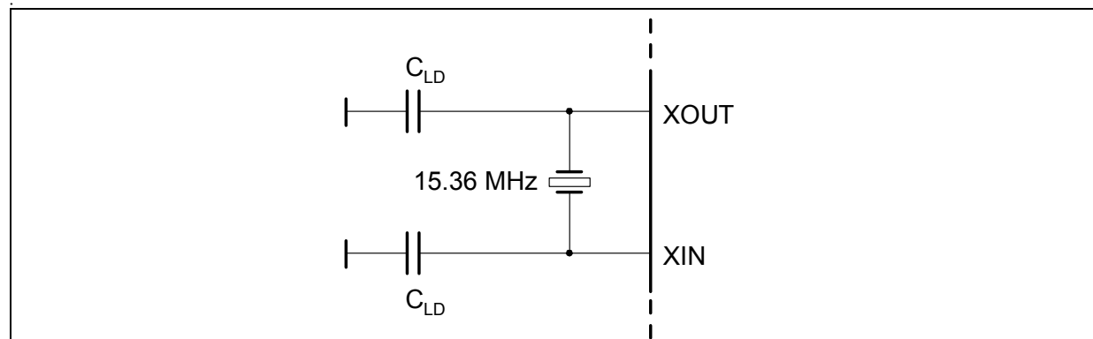
Figure 66 Crystal Oscillator
