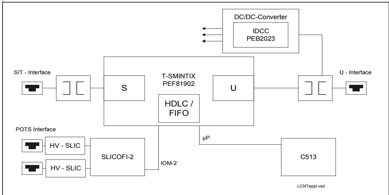
Figure 3 Application Example T-SMINT®IX: Low Cost Intelligent NT
