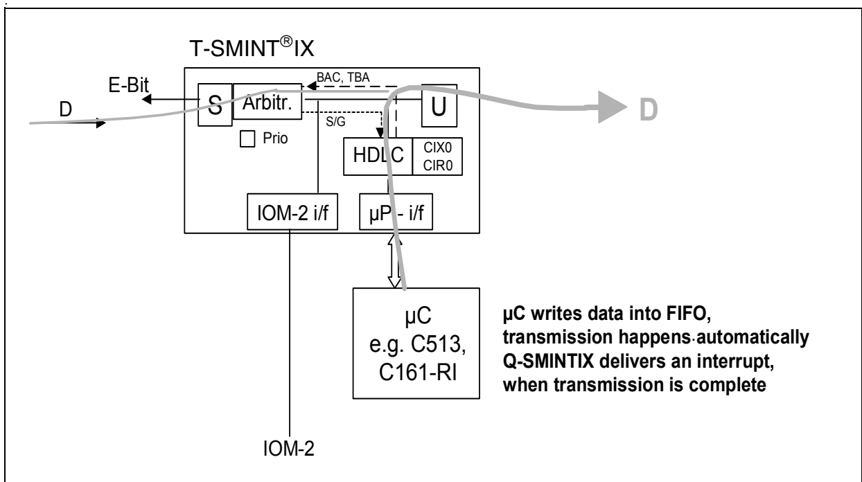
Figure 26 D-Channel Arbitration: \mu C has no HDLC and no Direct Access to TIC Bus
