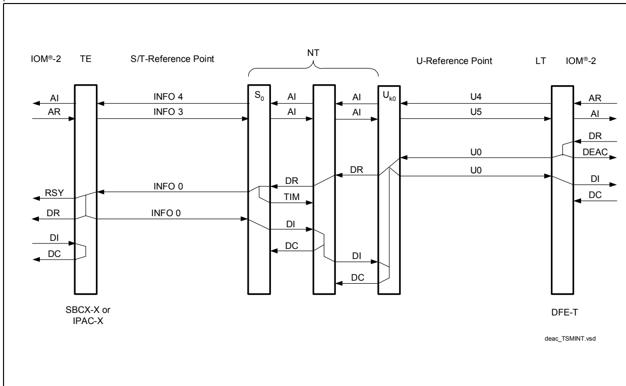
Figure 56 Complete Deactivation
