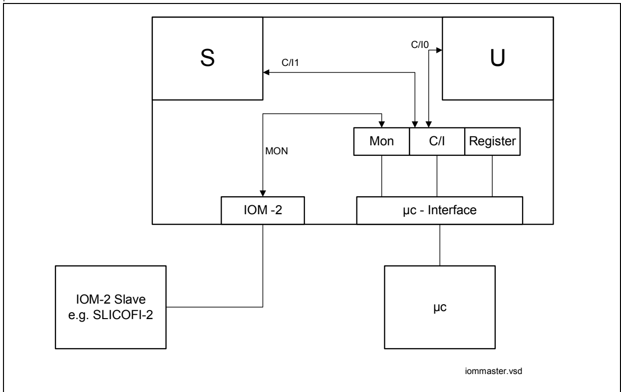
Figure 4 Control via \mu P Interface
