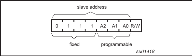
Figure 5. PCA9554A address
