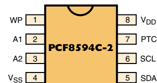
512 x 8-bit (4K) EEPROM
